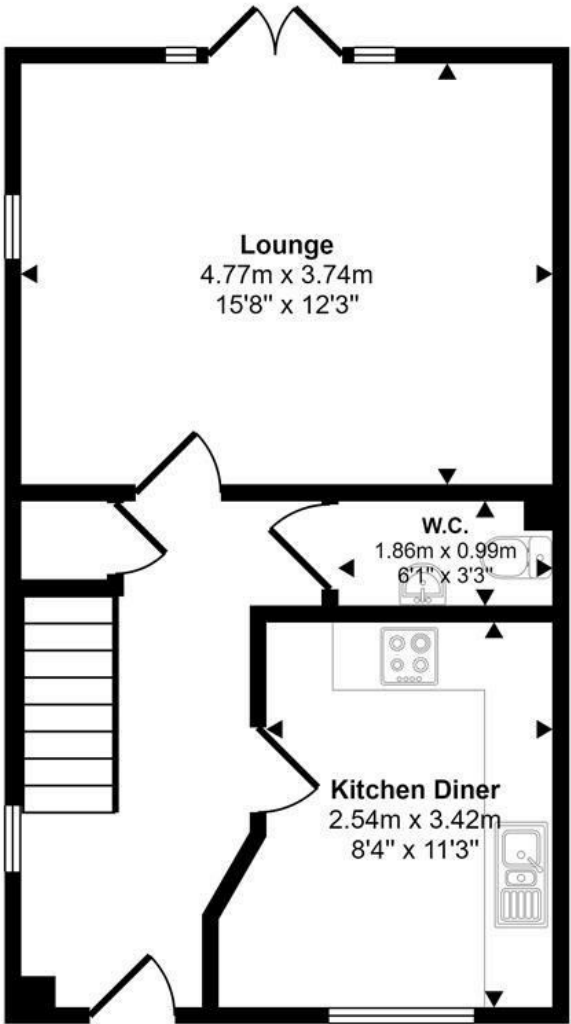
Ground Floor Approx 40 sq m / 429 sq ft
